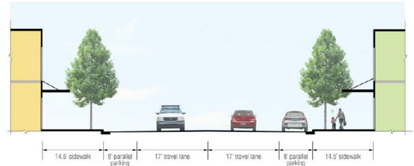
W LEWIS STREET - EXISTING SECTION
