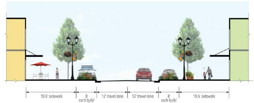
W LEWIS STREET - PROPOSED SECTION
